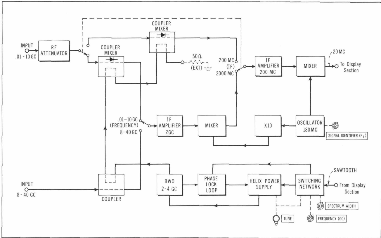
Fig. 5. Block diagram of Spectrum Analyzer RF Section. Only two inputs are needed to cover entire 0.01 to 40 Gc frequency range. Newly-developed RF attenuator does not require sepa-
