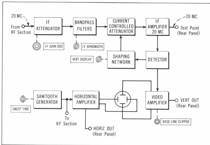
Fig. 6. Block diagram of Spectrum Analyzer Display Section.
