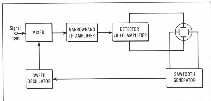
Fig. 3. Simplified block diagram of wide-band spectrum analyzer.
